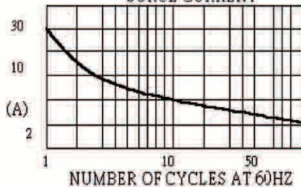
MAX. REPETITIVE FORWARD SURGE CURRENT
