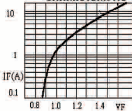
TYPICAL FORWARD CHARACTERISTIC
